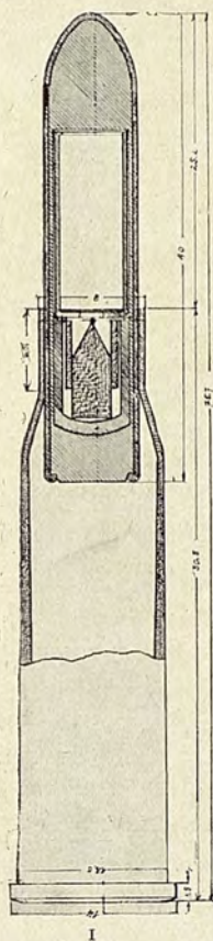
PLATE 2.—1. SKETCH OF A CARTRIDGE WITH EXPLOSIVE BULLETS; 2. CHAMBER FOR POWDER; 3. BASE OF THE CASE BEARING THE DATE 1912 AND THE AUSTRIAN EAGLE; 4. GUIDE TUBE; 5. STRIKER; 6. CHAMBERS FOR NOS. 4 AND 5.
