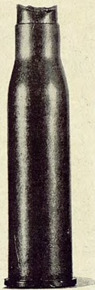
PLATE 2.—1. SKETCH OF A CARTRIDGE WITH EXPLOSIVE BULLETS; 2. CHAMBER FOR POWDER; 3. BASE OF THE CASE BEARING THE DATE 1912 AND THE AUSTRIAN EAGLE; 4. GUIDE TUBE; 5. STRIKER; 6. CHAMBERS FOR NOS. 4 AND 5.
