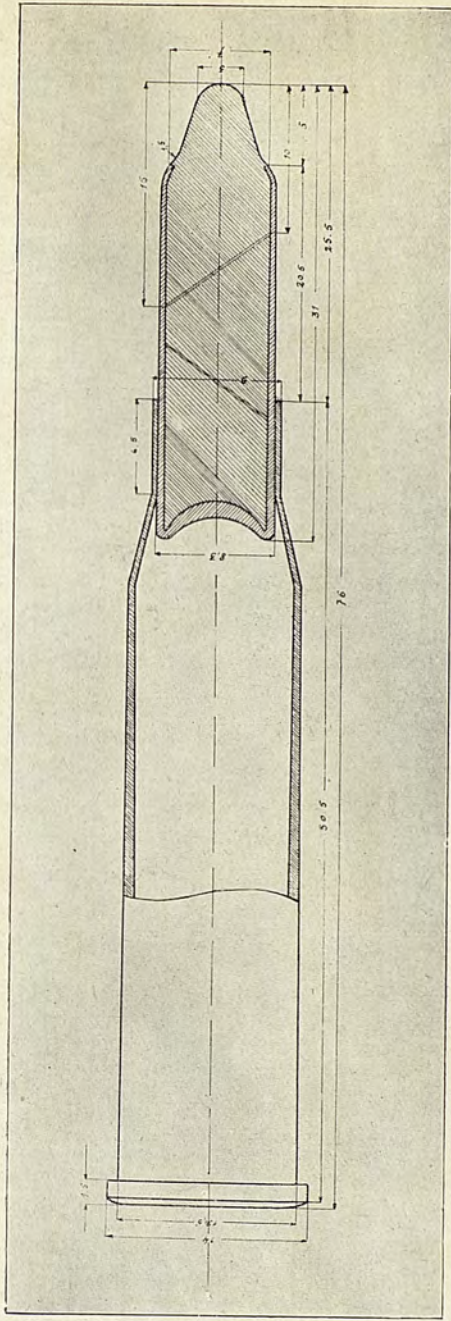
PLATE II.—SECTION OF AN AUSTRIAN EXPANDING CARTRIDGE (DUM-DUM). See page 16.
