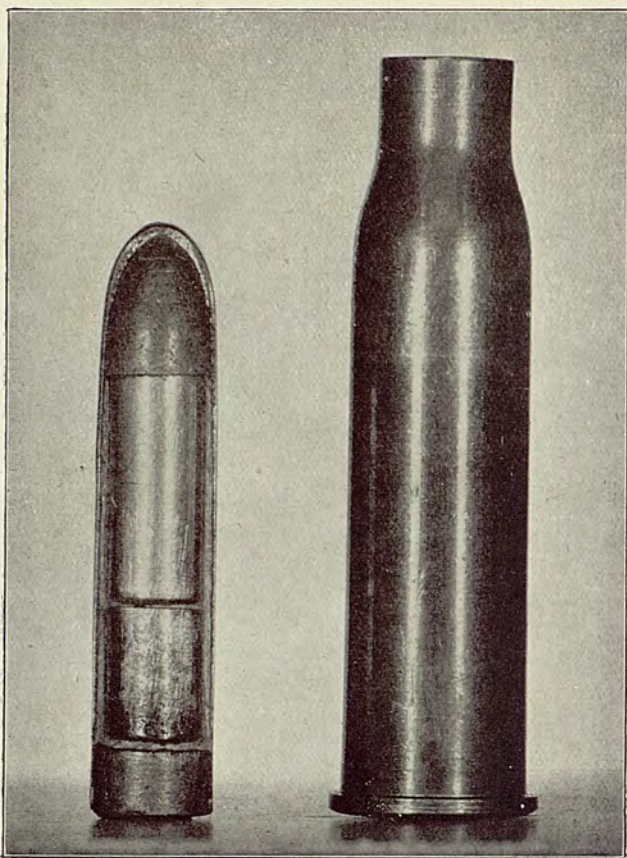
PLATE 5.—SECTION OF AN AUSTRO-HUNGARIAN EXPLOSIVE CARTRIDGE.
