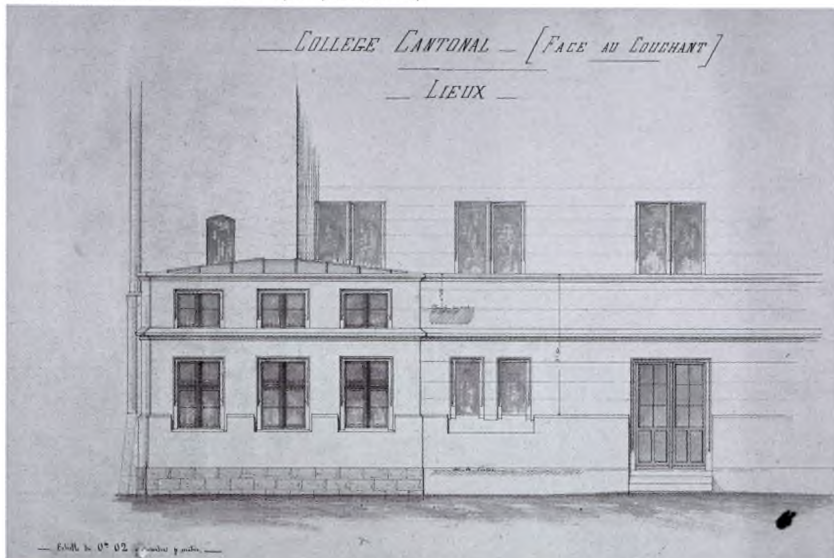
College cantonal. Dessin technique. (ACV, Bm 9).
